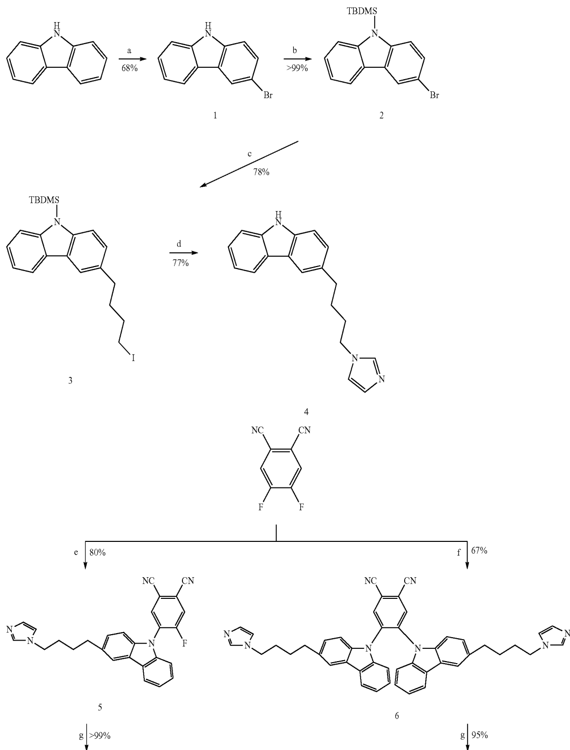
Scheme A. Synthesis of charged TADF emitters.
